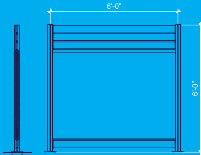
FENCE. FRONT VIEW
