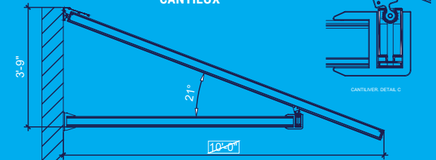
CANTILIVER, MAX ANGLE
